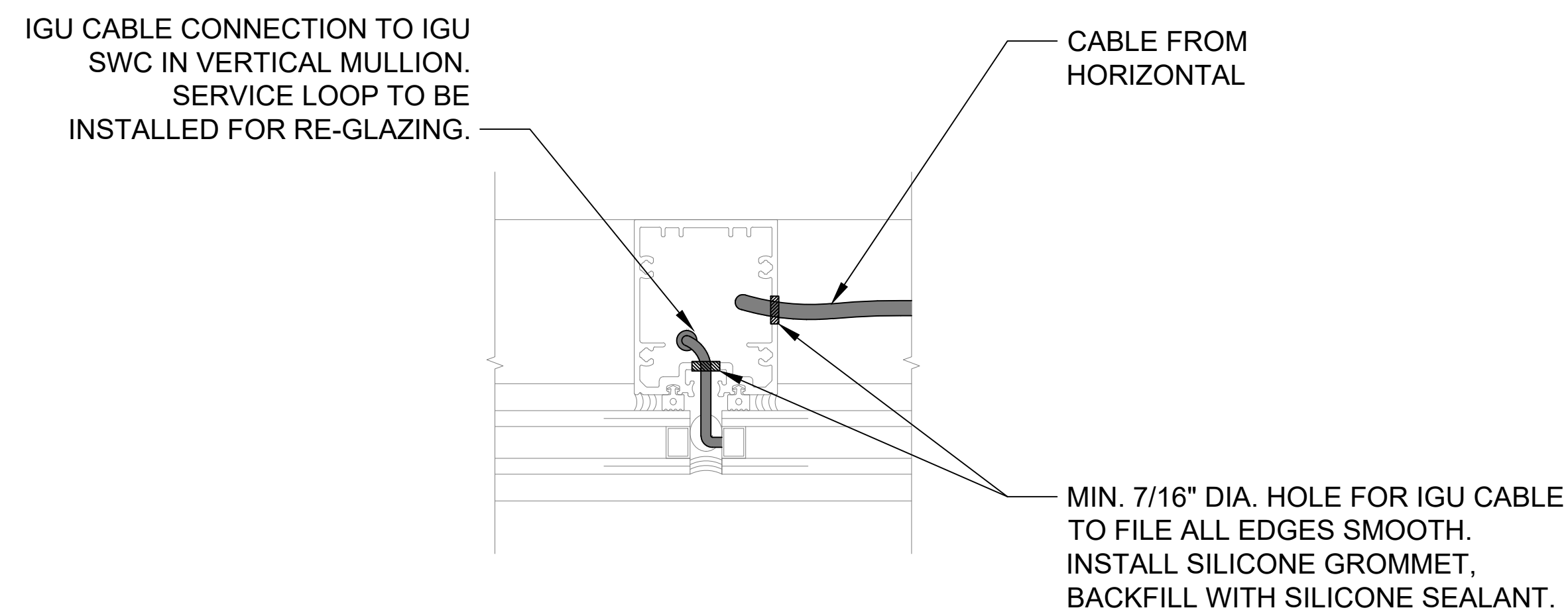
DETAIL 5 VERTICAL MULLION
